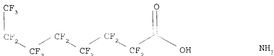
Compound (2) :
