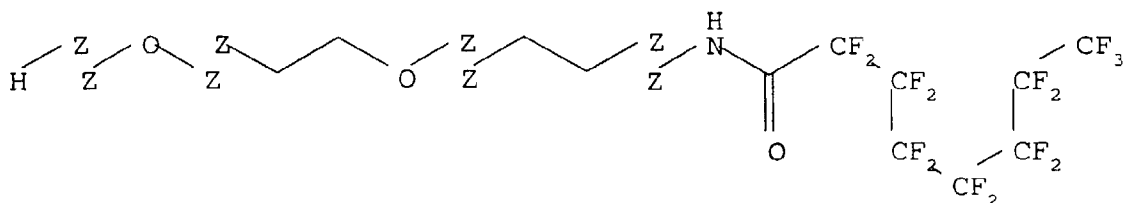
Compound (3) :
