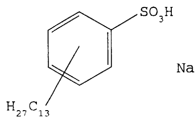
Compound (4) :
