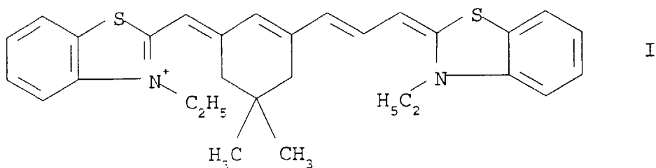
Sensitising Dye (2):
