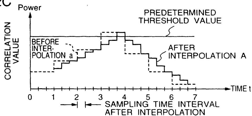
COMPARATOR OUTPUT USING INTERPOLATION VALUE
