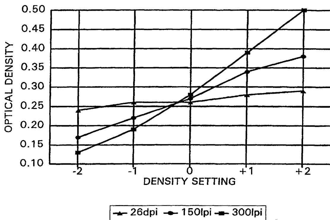
SENSITIVITY VS. DOTS/LINES PER INCH FIG. 2
