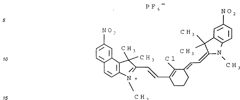
20 2-(2-(2-chloro-(3-(1,3-dihydro-1,3,3-trimethyl-5-nitro-2H-indol-2-ylidene)ethylidene)-1-cyclohexene-1-yl)ethenyl)-1,3,3-trimethyl-5-nitro-3H-indolium hexafluorophosphate
