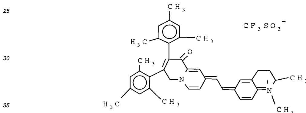
40 2,3,4,6-tetrahydro-1,2-dimethyl-6-[[1-oxo-2,3-bis(2,4,6-trimethylphenyl)-7(1H)-indolizinylidene]ethylidene]quinolinium trifluoromethanesulfonate.
