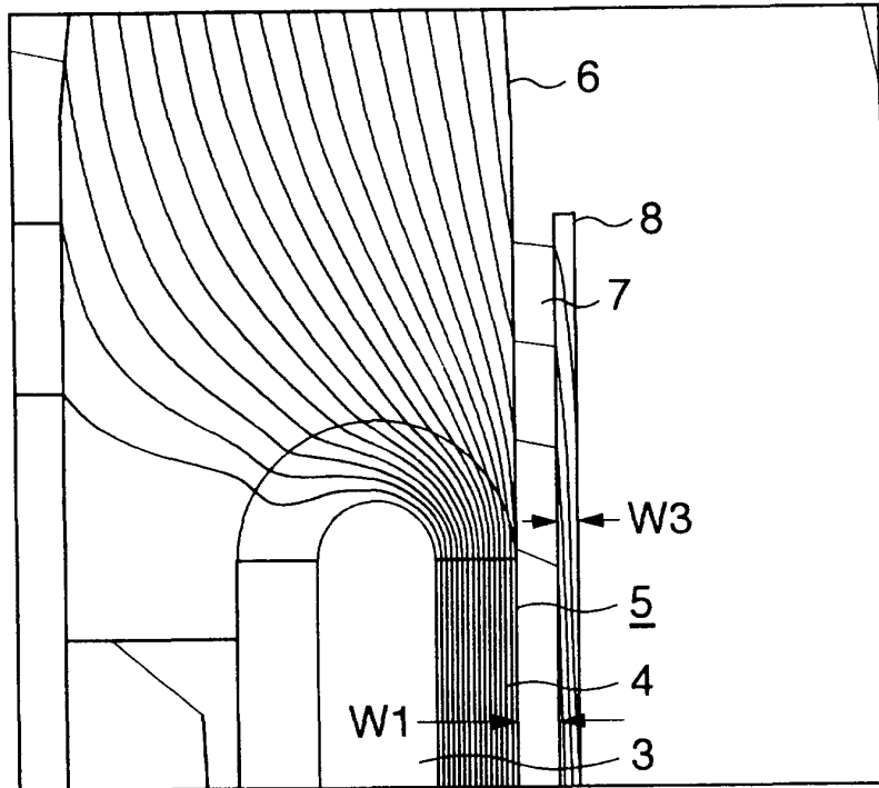
FIG. 4 PRIOR ART
