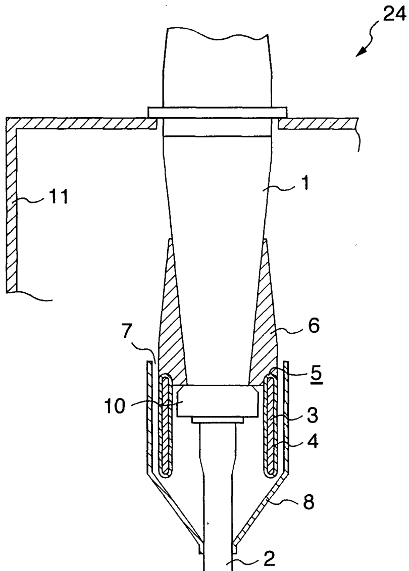
FIG. 2 PRIOR ART
