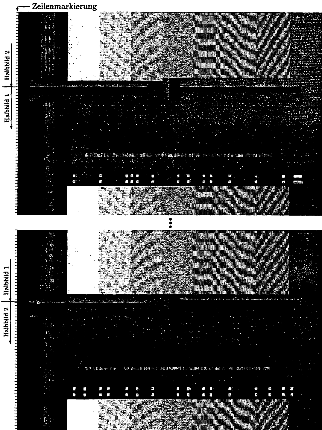
Fig. 6: Videosequenz, Vertikal-Synchronsignal
