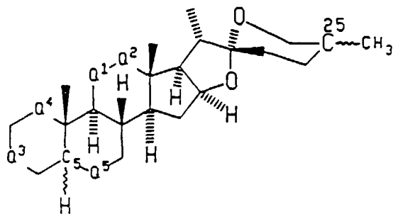
Formula IA
