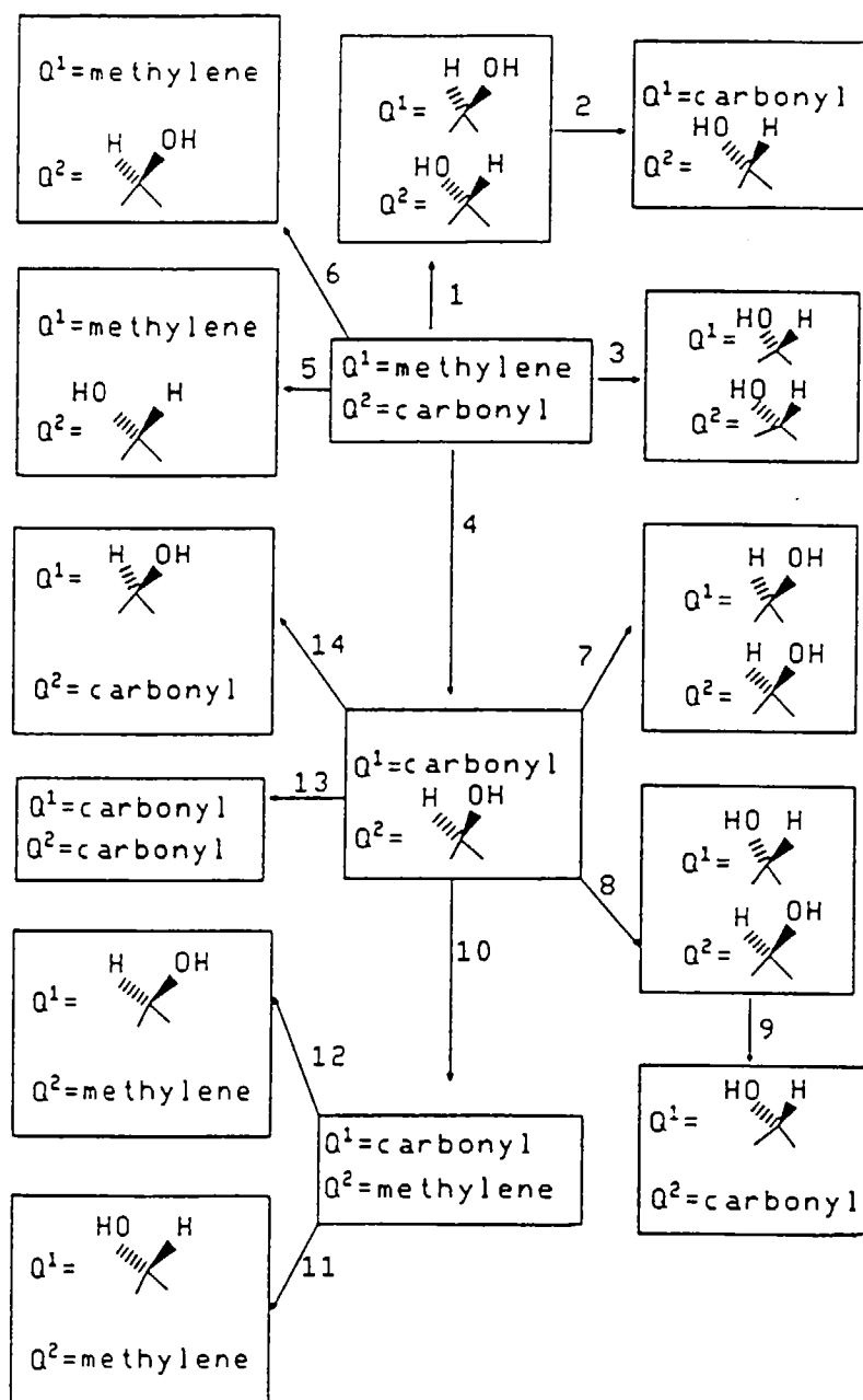
SCHEME IV
