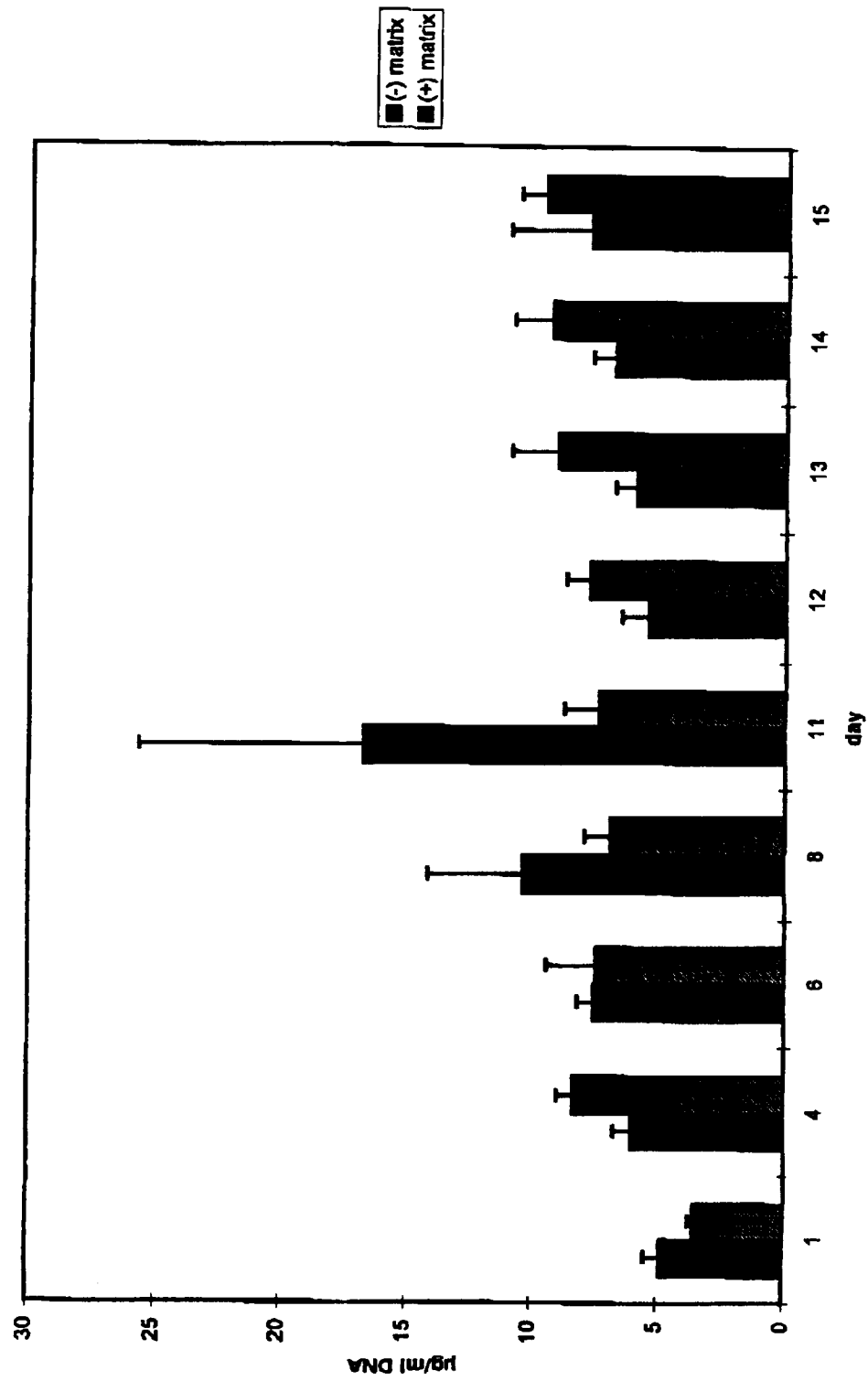
Figure 6a. DNA content U96092
