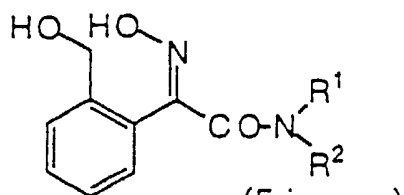
(E-isomer) ( I-1 )
