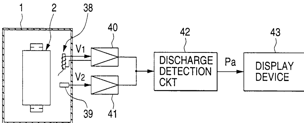
FIG. 13 PRIOR ART
