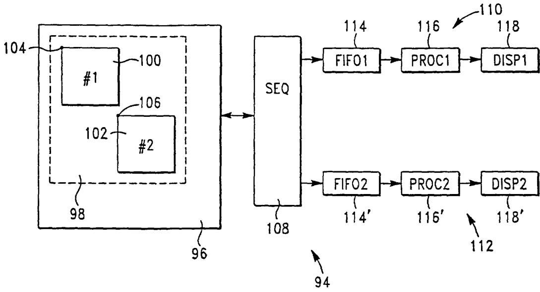
FIG.-13 (PRIOR ART)
