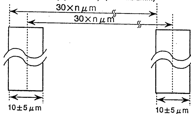
Fig. 5b Slit Dimension Accuracy (Precision) (at r=22.2\text{mm} )
