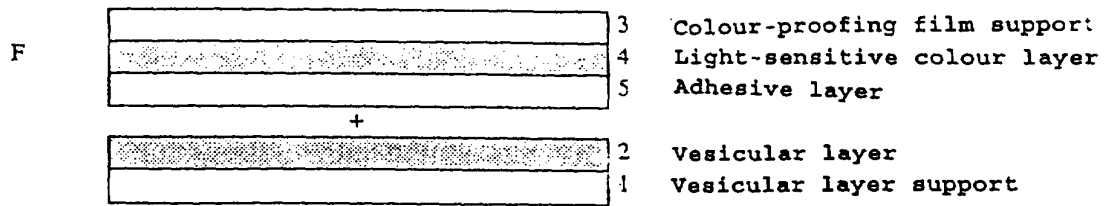
Fig. 1 Construction of the image support of the invention and of the 1st colour-proofing film F before lamination
