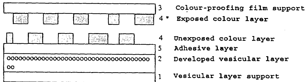
Fig. 3 Construction of coloured image of the invention after development of 1st primary colour image
