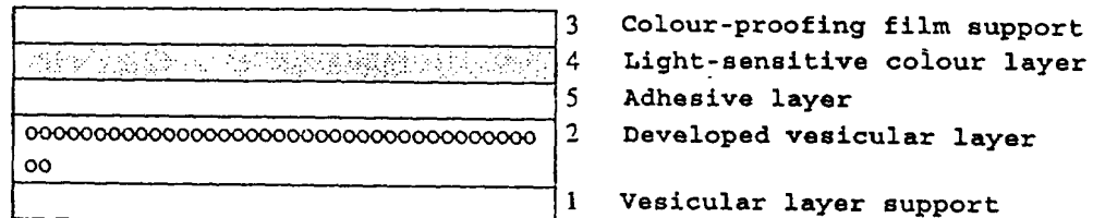
Fig. 2 Construction of coloured image of the invention following lamination of the 1st primary colour
