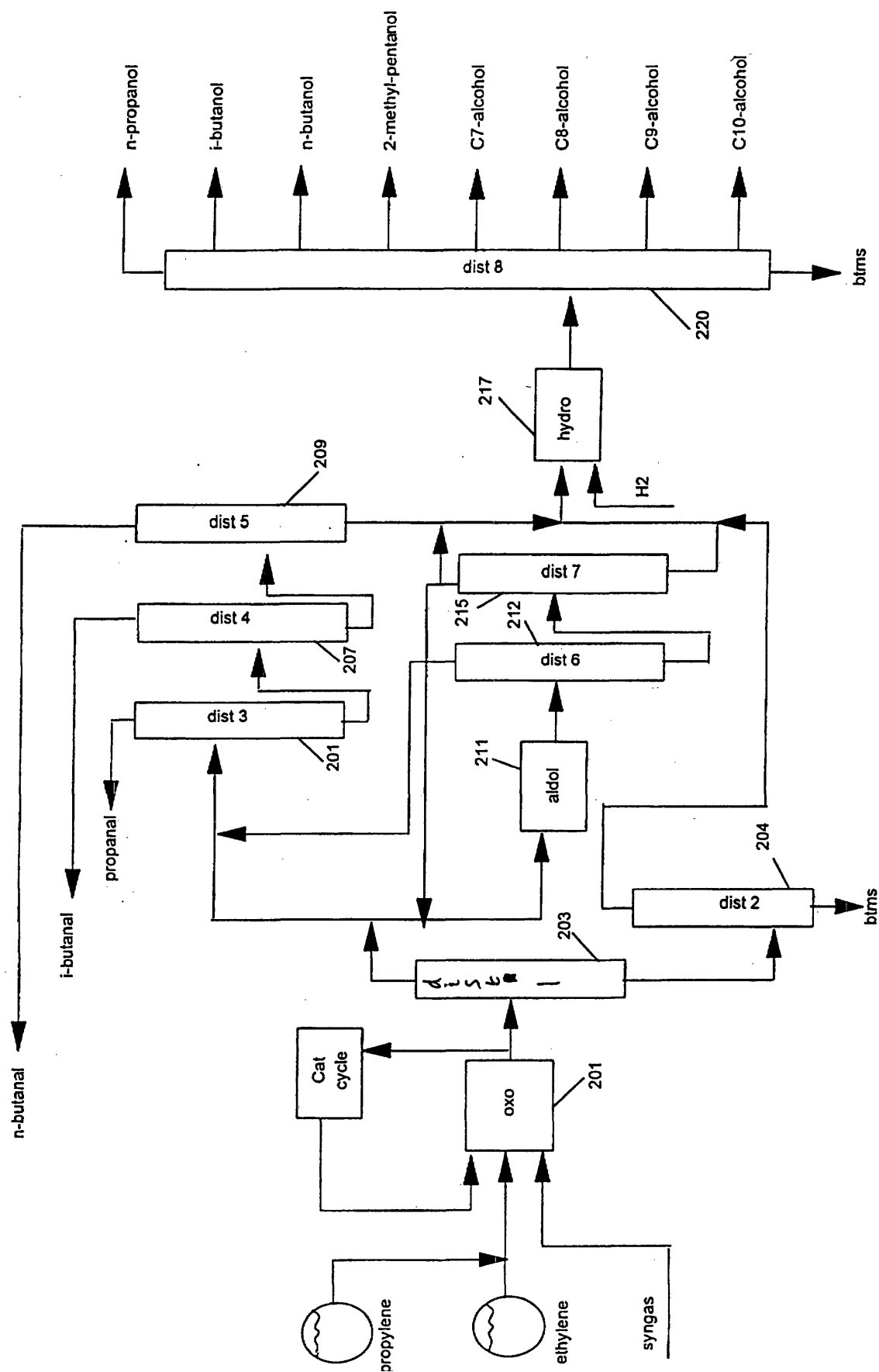
Figure 5. Ethylene/Propylene Cofeeding to Produce C3-C10 Alcohols and Light Aldehydes
