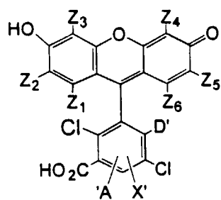
4,7 Dichlorofluorescein (See Pat. No. 5,188,934)
