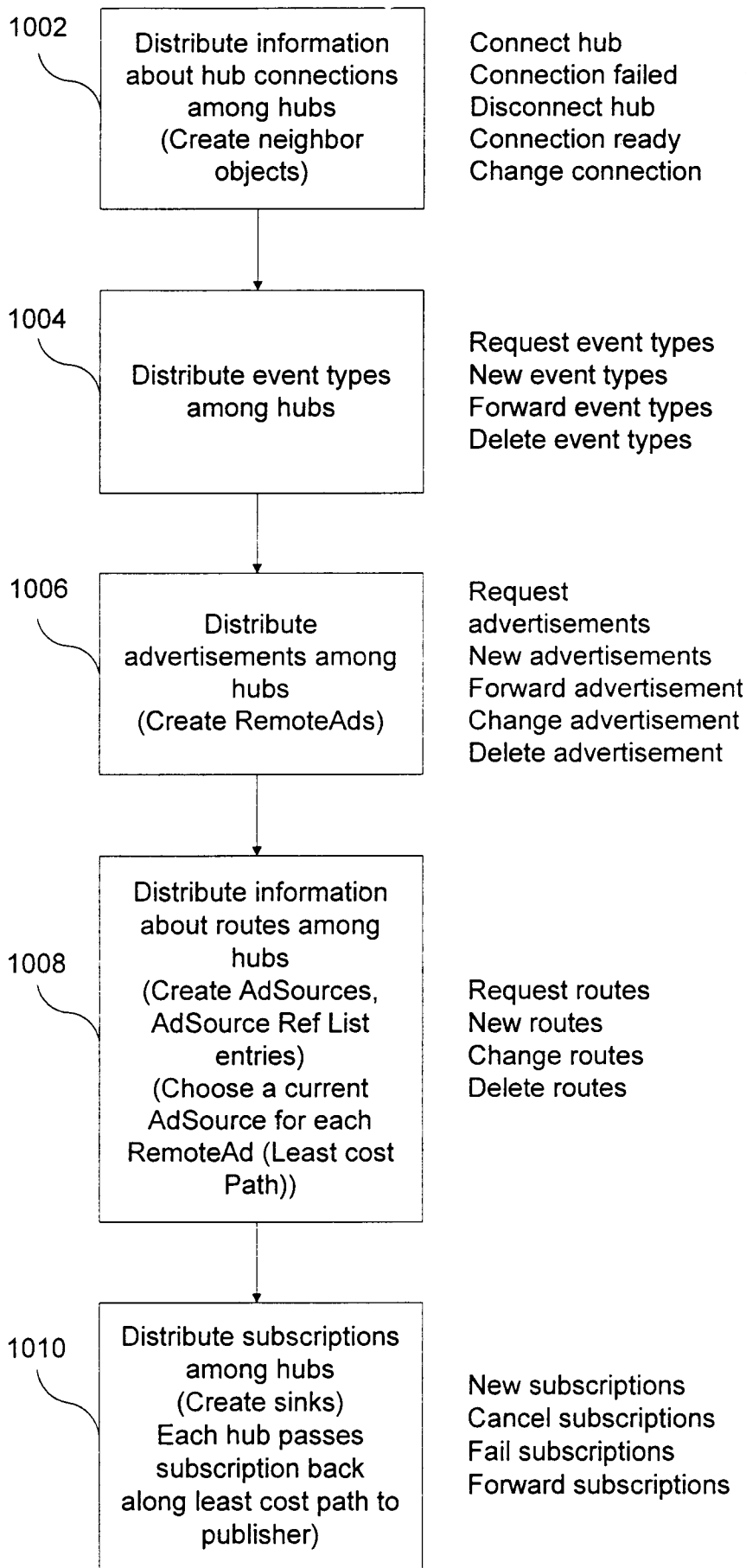
FIG. 10 Populating Data Structures of Hubs
