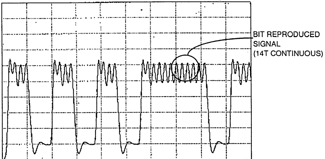
(b) SIMULATOR WAVEFORM AFTER LPF : I_{14L} = I_S = 0.1
