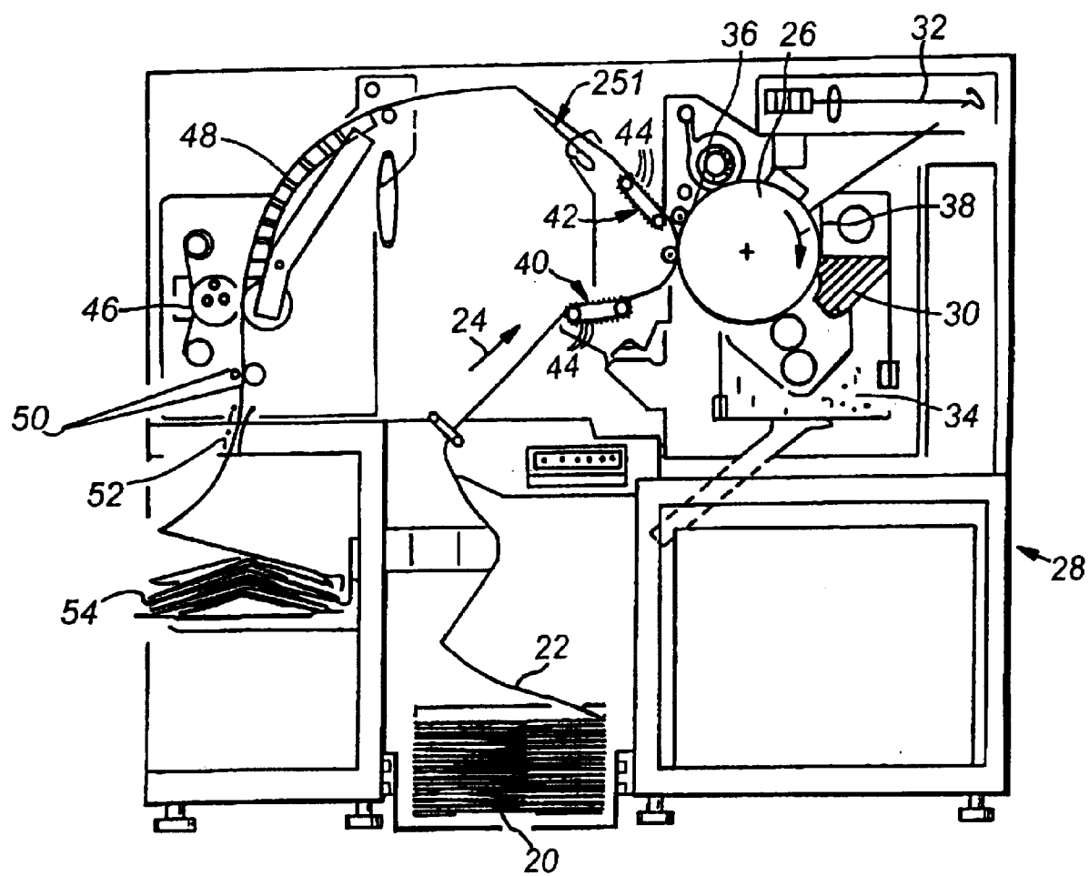
FIG.2 (PRIOR ART)
