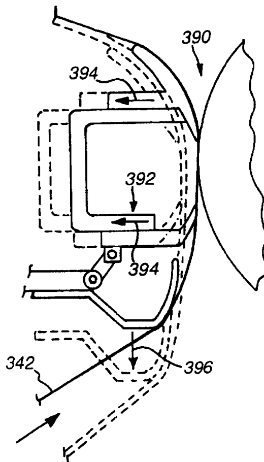
FIG. 16 (PRIOR ART)
