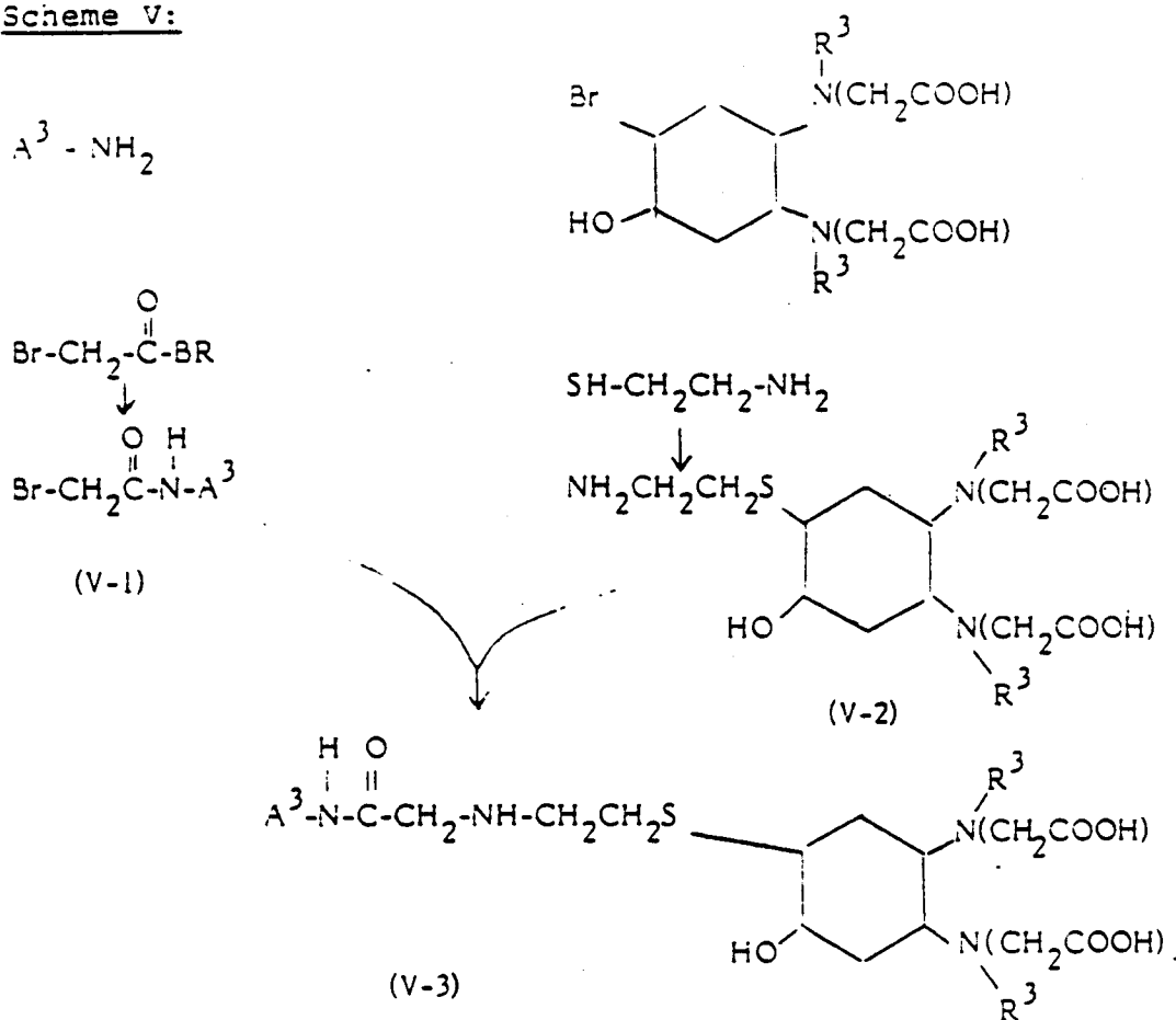
Scheme V:
