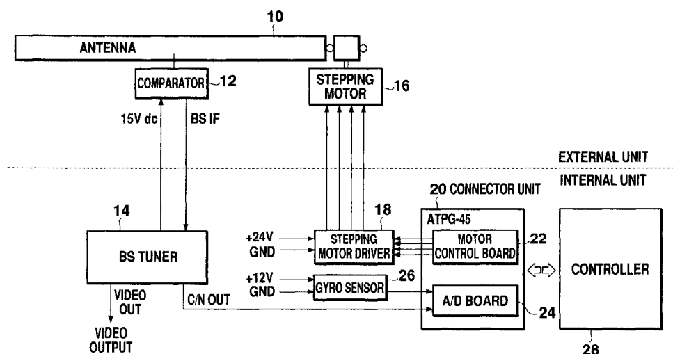
BLOCK DIAGRAM OF BS TRACKING SYSTEM
