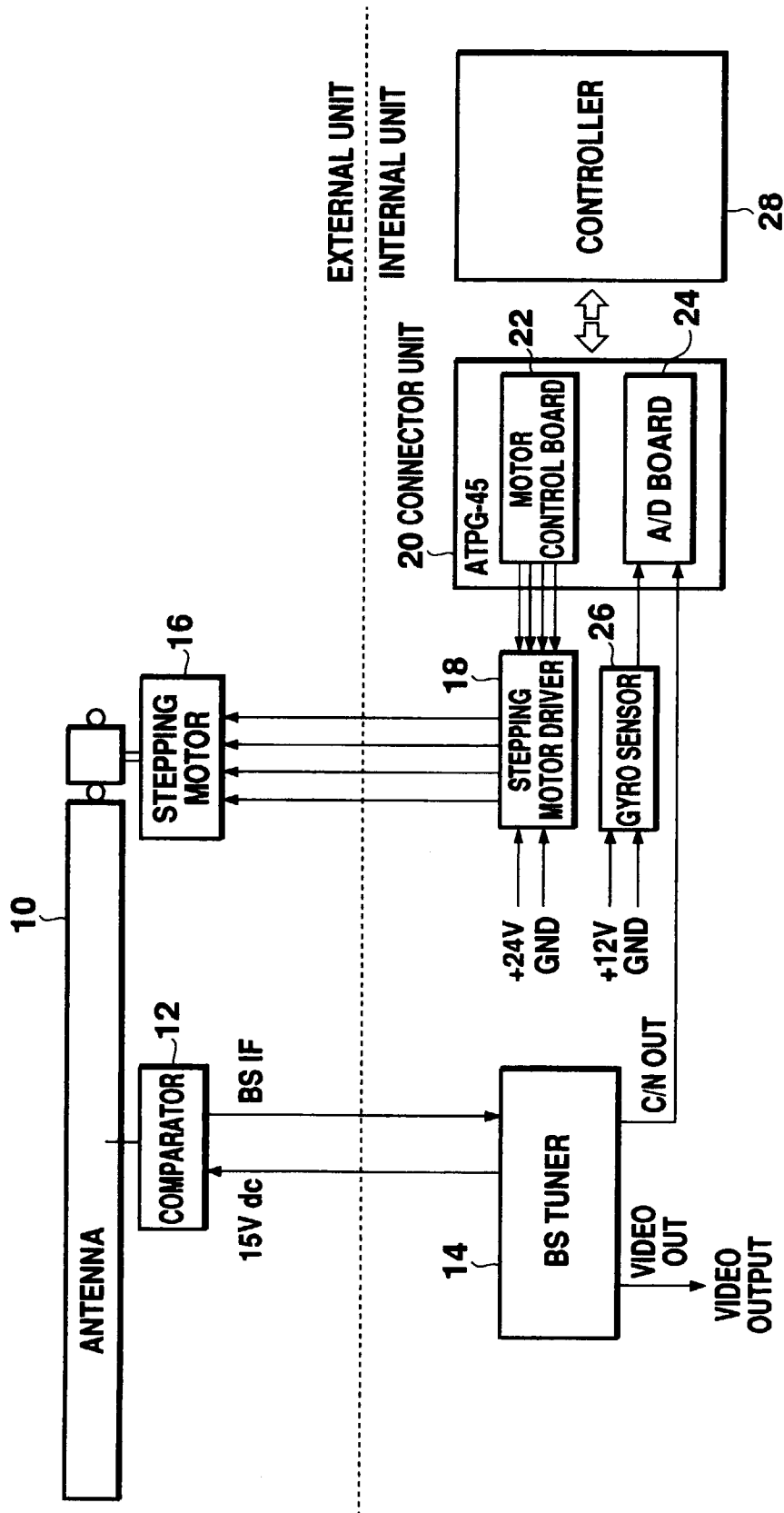
BLOCK DIAGRAM OF BS TRACKING SYSTEM
