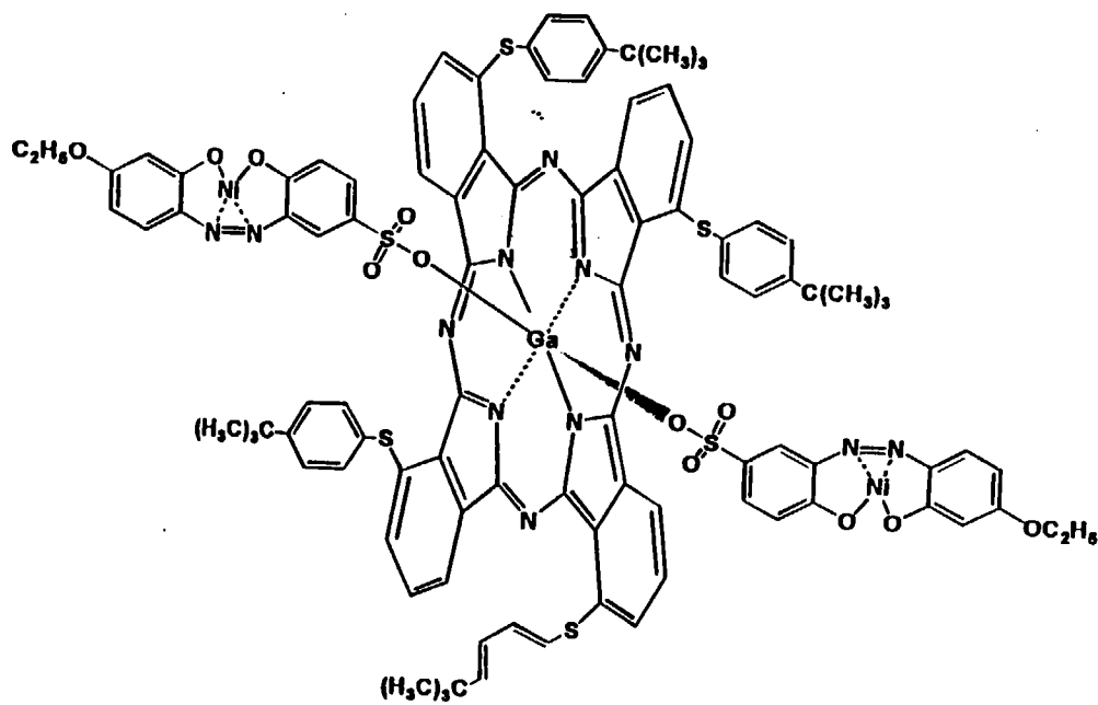
Phthalocyanine compound (n)
