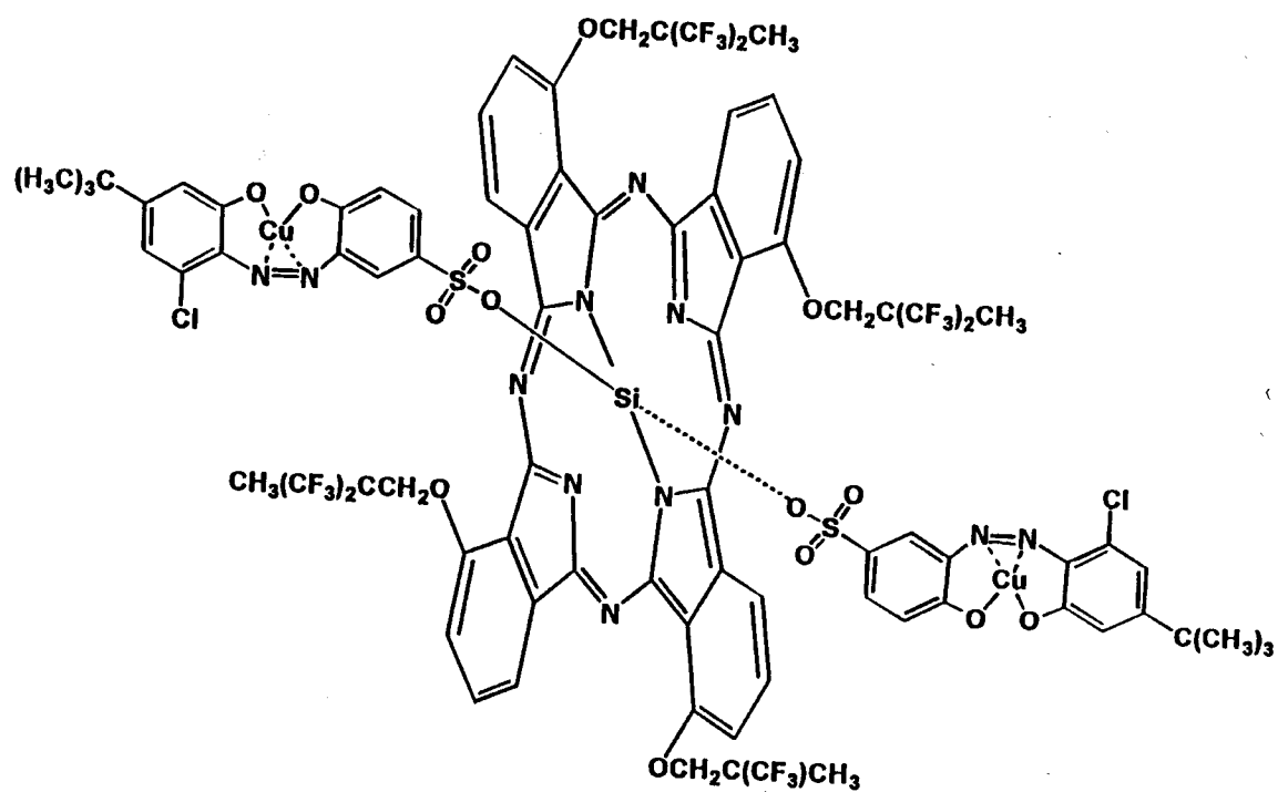
Phthalocyanine compound (f)
