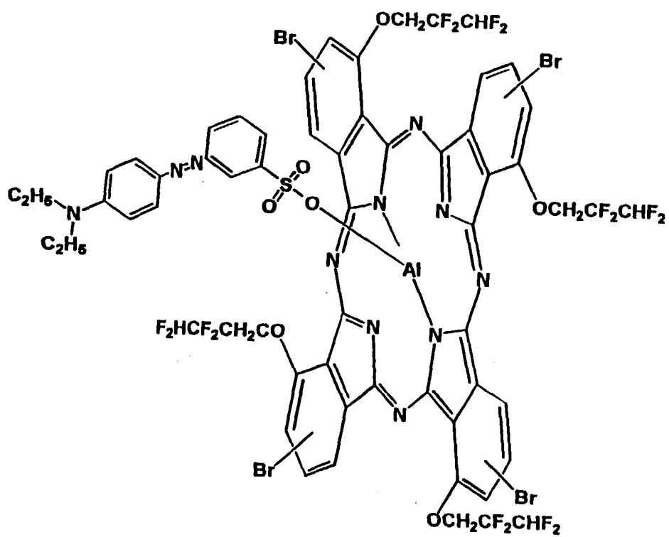
Phthalocyanine compound (b)
