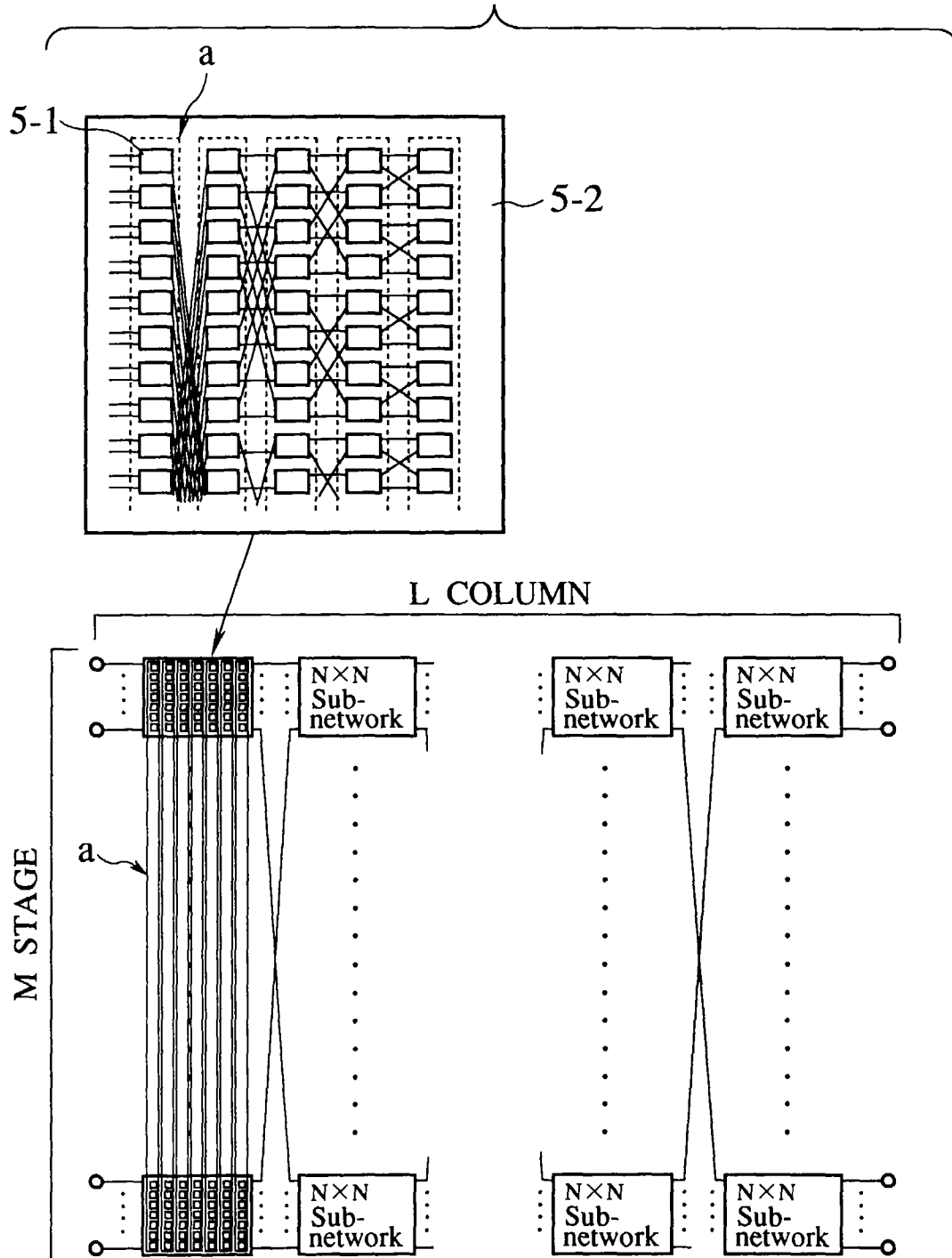
FIG.5 PRIOR ART
