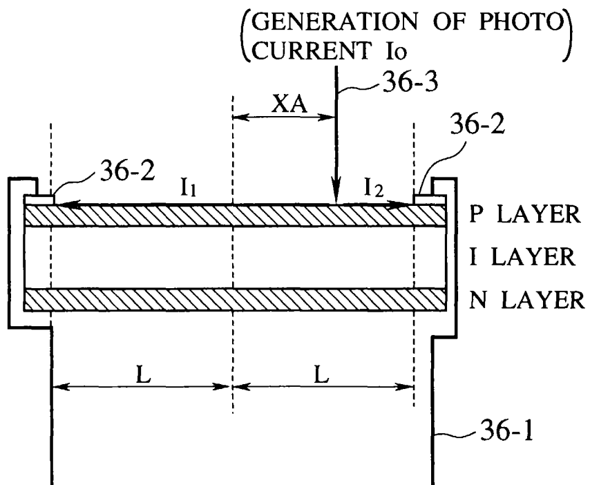
FIG.36B
