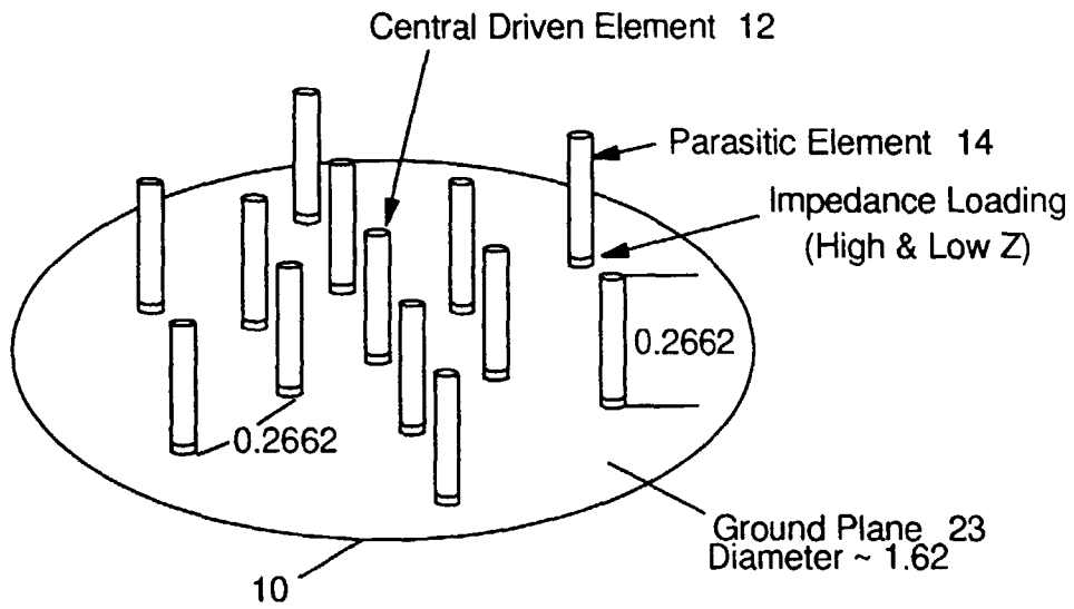
Parasitic Monopole Array
