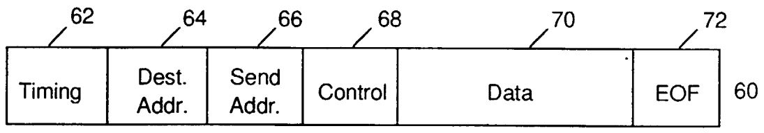
Transmission Packet
