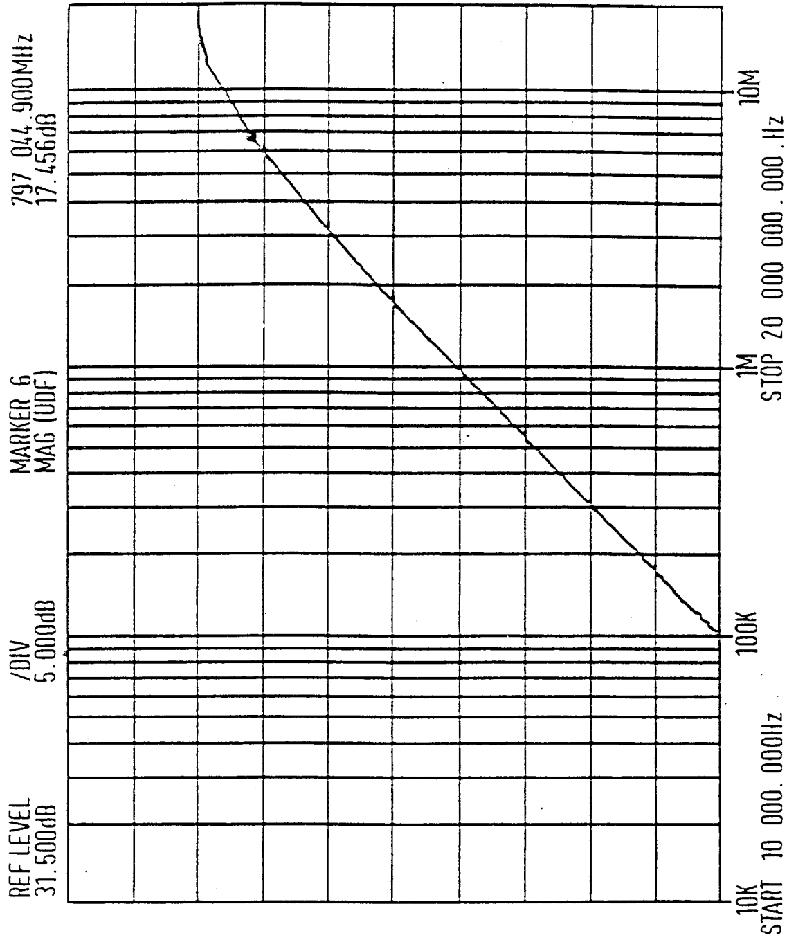
FIG. 14A DIFFERENTIATOR
