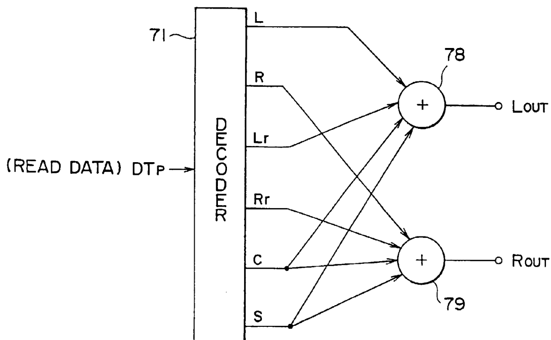
6-ch DATA REPRODUCTION IN 2-ch MODE
