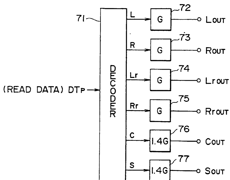
6-ch DATA REPRODUCTION
