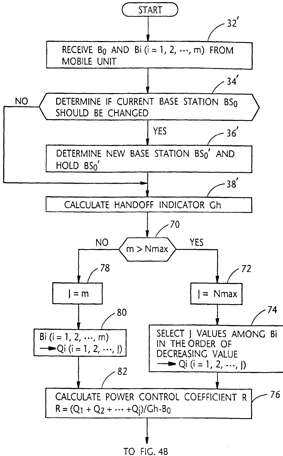
FIG. 6 AT CURRENT BASE STATION
