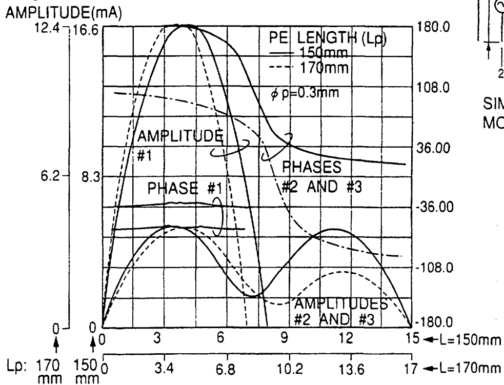
Fig. 4(b) CURRENT DISTRIBUTIONS FOR DIFFERENT PE LENGTHS
