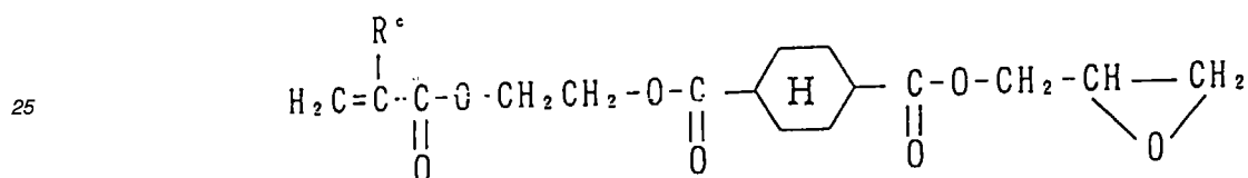
30 2-(meth)acryroyloxyethylhexahydro terephthalic acid glycidylester
