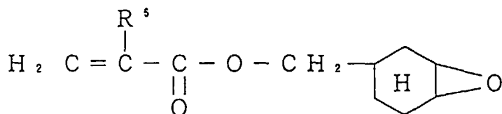
3,4-epoxyhexahydrobenzyl (meth)acrylate
