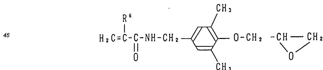
50 4-glycidyoxy-3,5-dimethylbenzyl(meth)acrylamide
