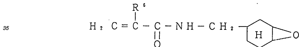
40 3,4-epoxyhexahydrobenzyl(meth)acrylamide
