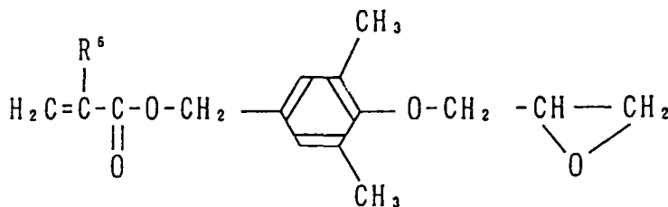
4-glycidyloxy-3,5-dimethylbenzyl (meth)acrylate
