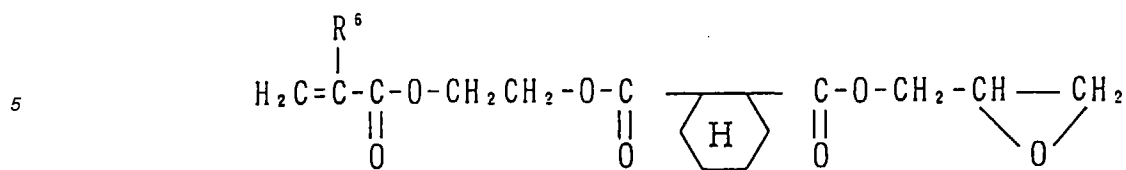
10 2-(meth)acryroyloxyethyl hexahydrophthalic acid glycidylester
