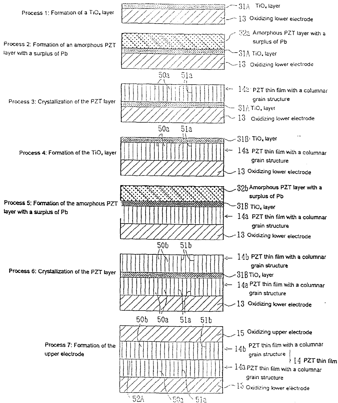
FIG. 2. A process for forming the PZT capacitor of this embodiment
