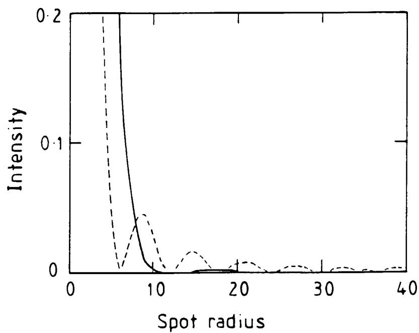
FIG 11f Diffracted spot intensity profile (from fast fourier transform)
