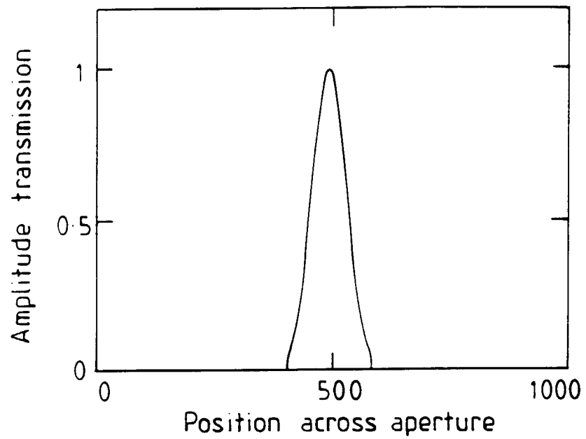
FIG 11i truncated gaussian Pixel aperture transmission function
