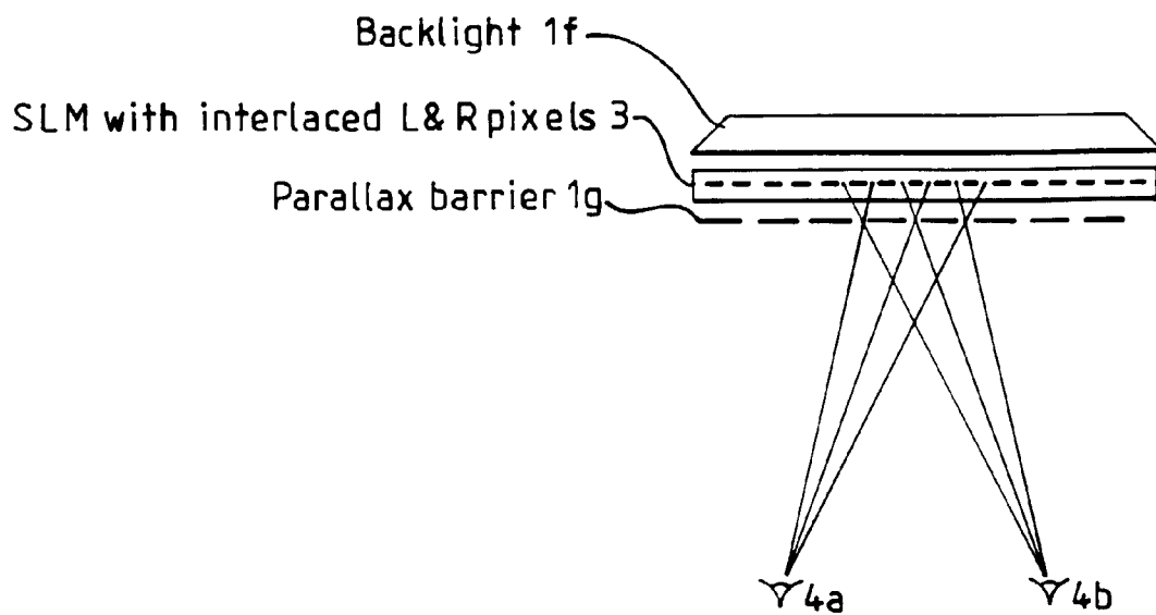
FIG 20 Front parallax barrier autostereoscopic display
