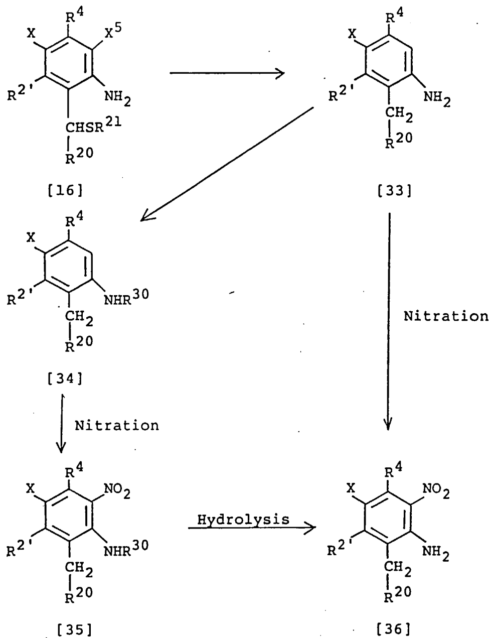
[Reaction scheme-X]
