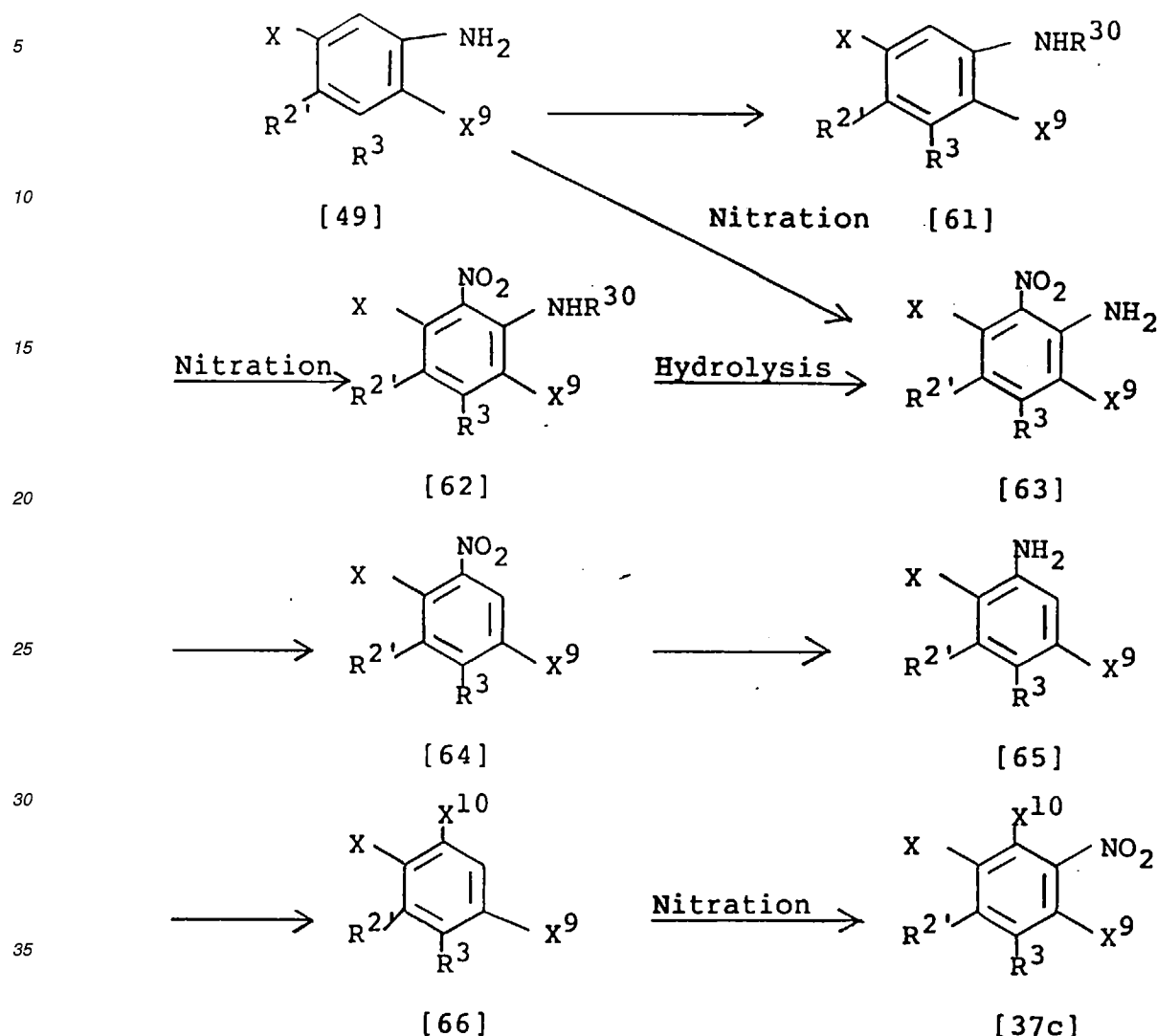
[Reaction scheme-XV]
