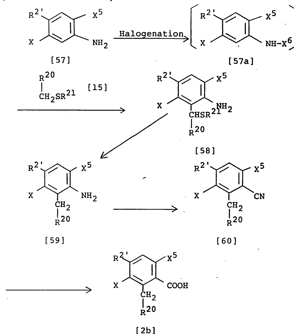
[Reaction scheme-XIV]
