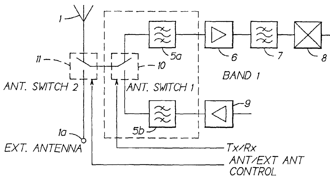
FIG. 9 PRIOR ART
