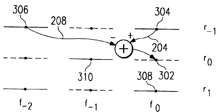
FIG. 3 (PRIOR ART)
