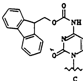
Cytosine (C)
