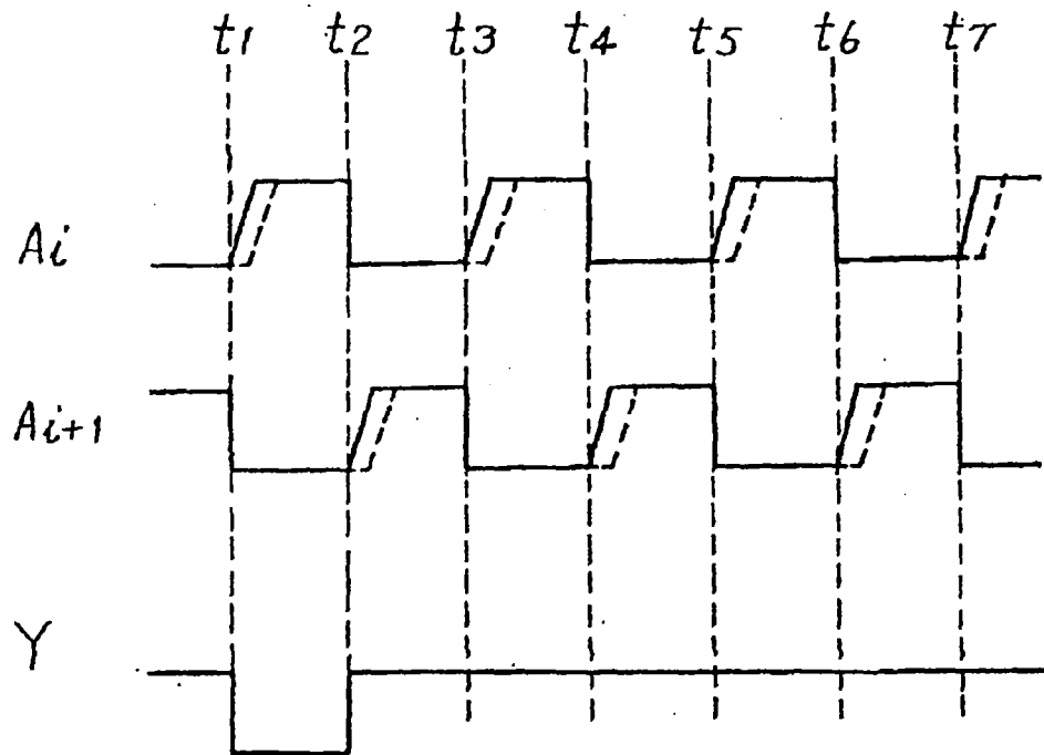
FIG. 22 WAVEFORM OF DRIVE PULSE EXAMPLE 5
