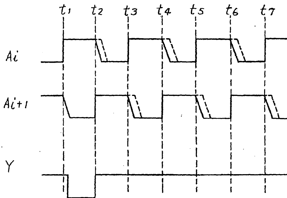
FIG. 23 WAVE OF DRIVE PULSE EXAMPLE 6
