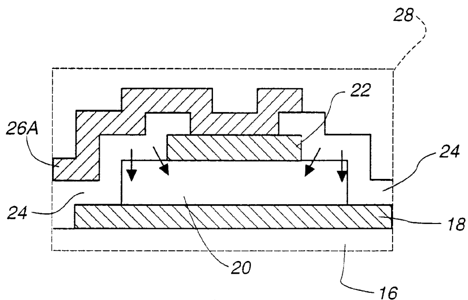
Fig. 2 Prior Art
