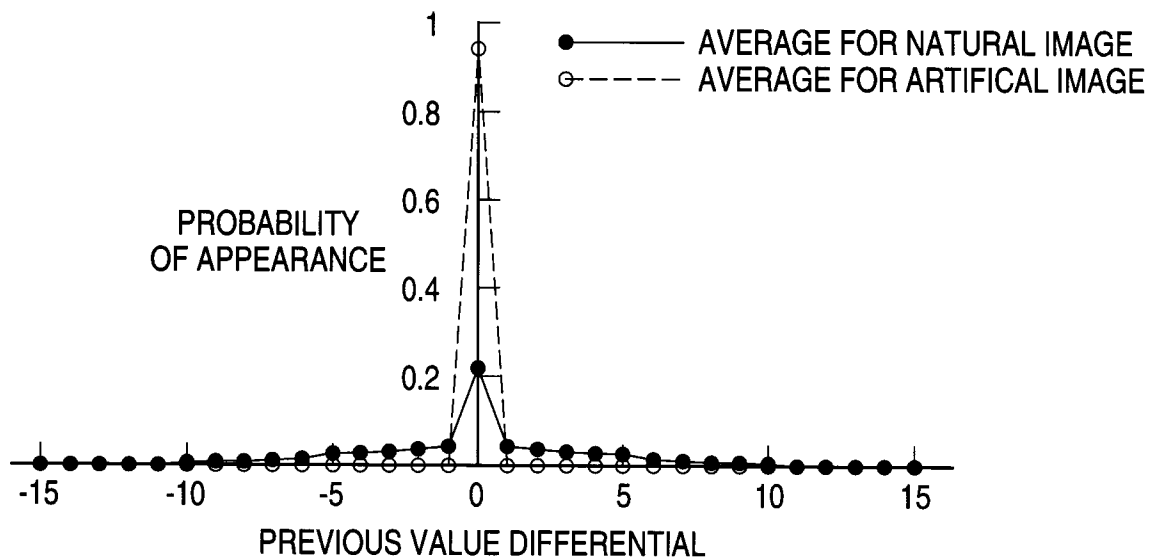
COMPARISON OF DISTRIBUTION OF PREVIOUS VALUE DIFFERENTIALS IN NATURAL IMAGES AND ARTIFICIAL IMAGES
