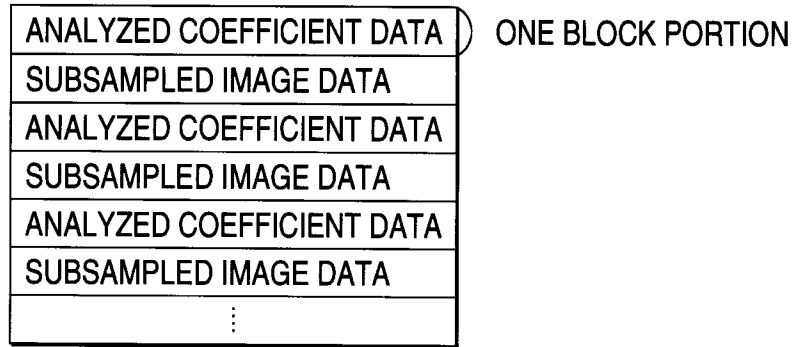
EXAMPLE 2 OF COMPOSITE DATA
