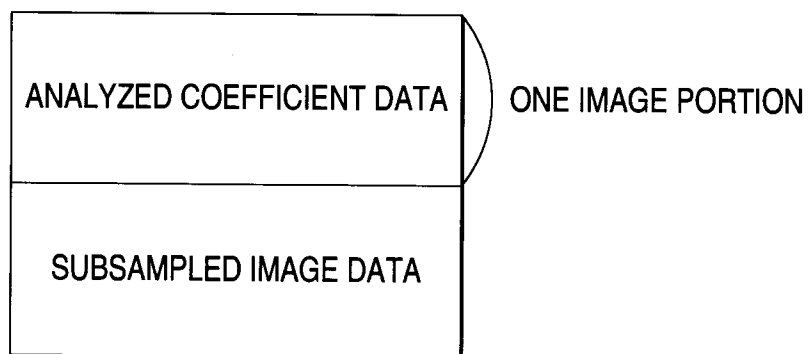
EXAMPLE 1 OF COMPOSITE DATA
