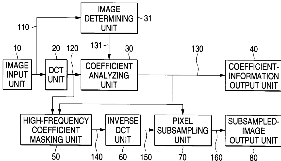
ENCODING APPARATUS FOR DYNAMICALLY CHANGING THRESHOLDS
