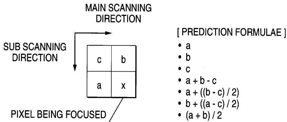
PREDICTION FORMULAE USED IN JPEG
