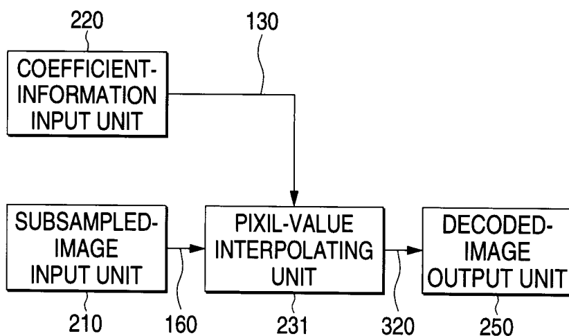
DECODING APPARATUS FOR DIRECTLY INTERPOLATING PIXEL VALUES
