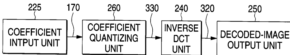
DECODING APPARATUS
