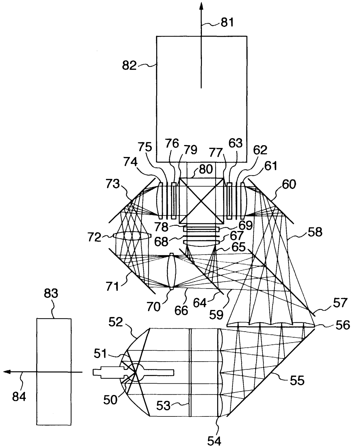
FIG. 9 PRIOR ART
