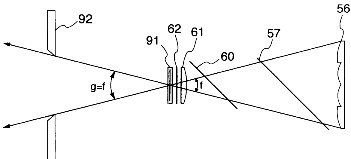
FIG. 11 PRIOR ART
