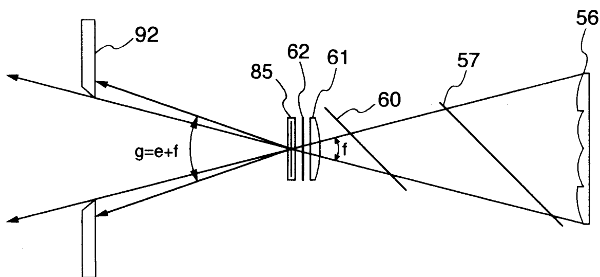
FIG. 12 PRIOR ART
