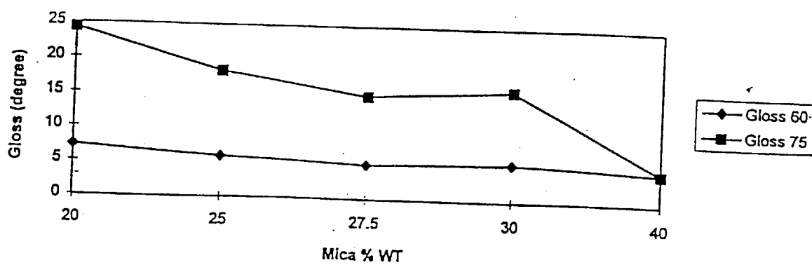
FIGURE 23 Gloss Versus Mica Level
