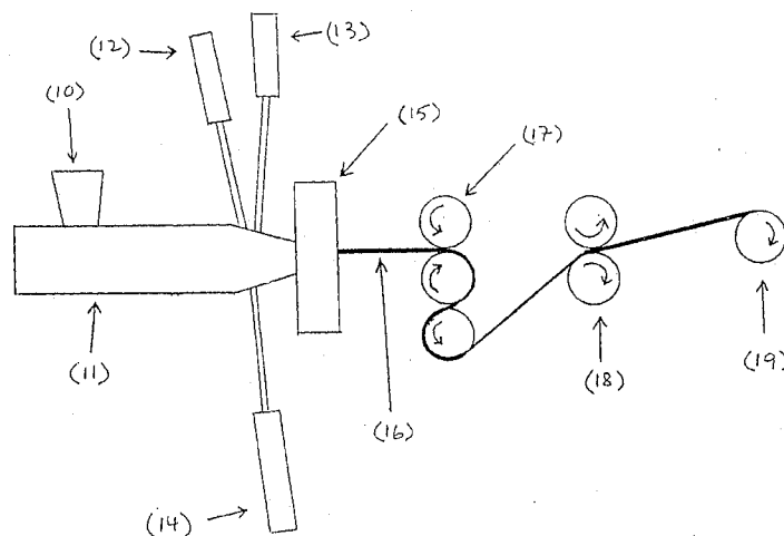
FIGURE 1 SHEET EXTRUSION PROCESS
