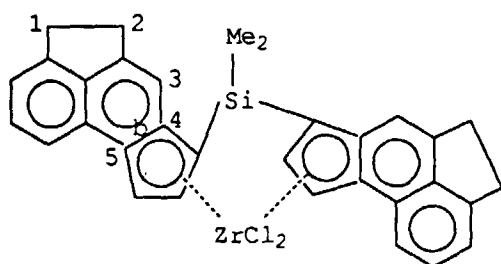
dimethylsilylene-bis(1,2- dihydroacenaphthyl[4,5- b]cyclopentadienyl) zirconium dichloride
