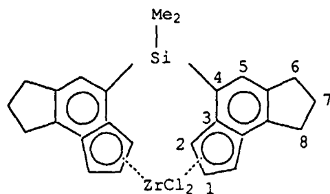
dimethylsilylene-bis(7,8- dihydro-3H,6H-3-as- indathenyl) zirconium dichloride
