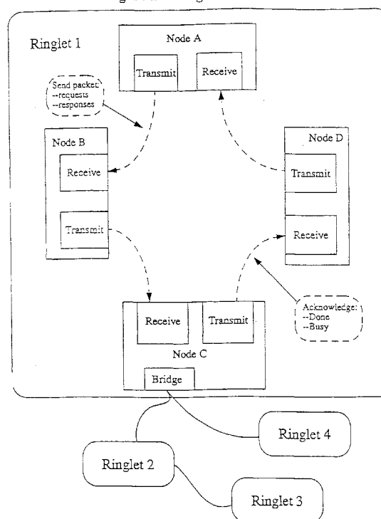
Figure 1 -- Ringlet/Network
