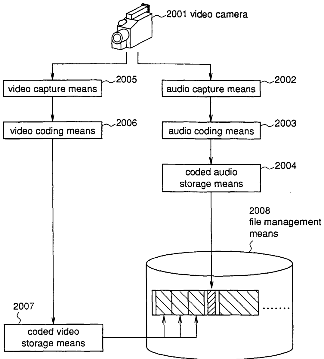
Fig.28 Prior Art
