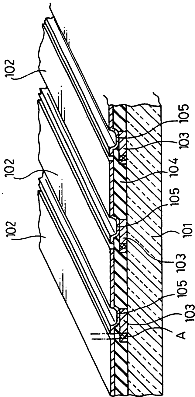
FIG. 24 PRIOR ART
