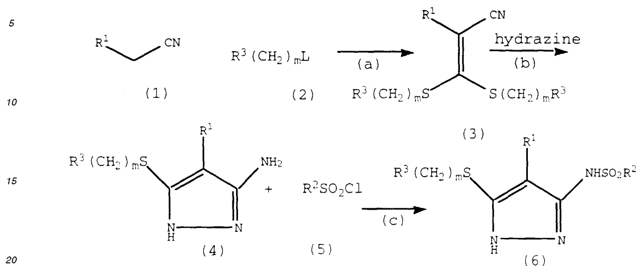
Scheme I
