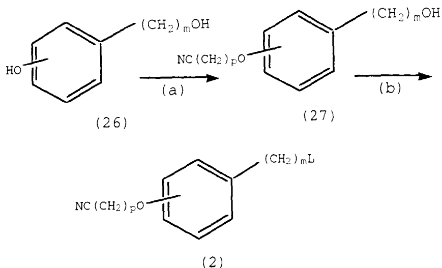
Scheme III(b)
