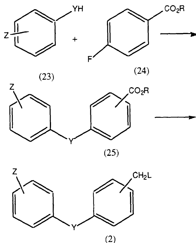
Scheme III(a)
