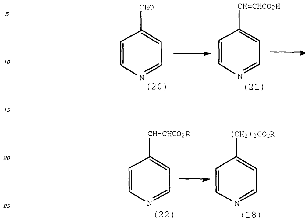
Scheme II (e)
