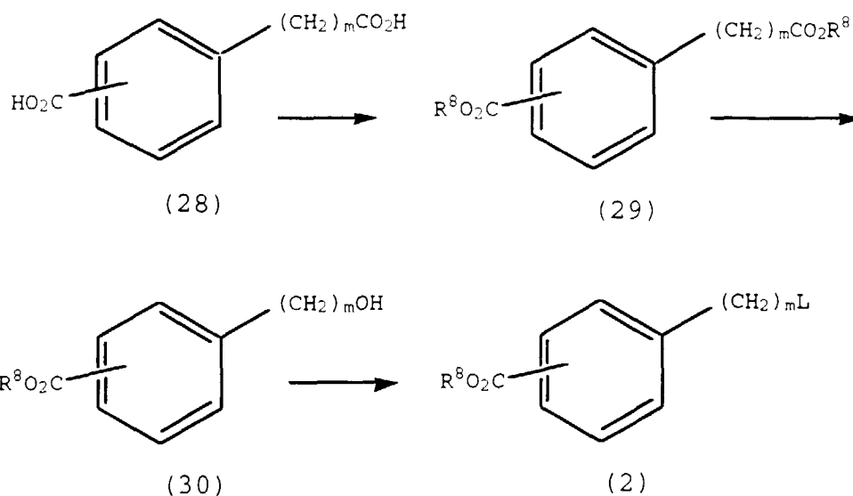
Scheme III(c)
