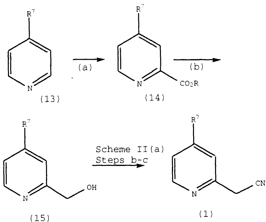
Scheme II(b)
