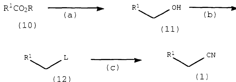
Scheme II (a)
