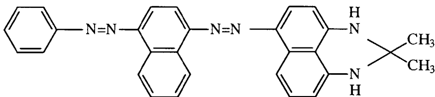
Sudan Black Dye
