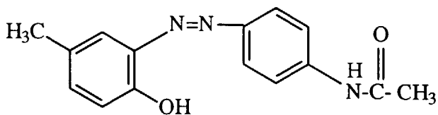
Keyplast Yellow Dye
