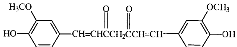
Curcumin Yellow Dye
