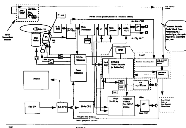
Block Diagram of DVD Player (ROM Type for Published Media) + TIRIS cypher
