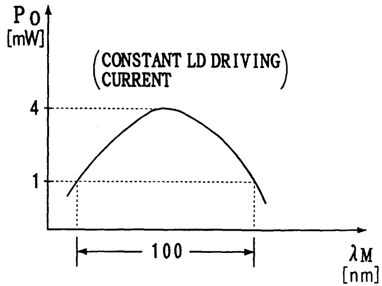
FIG.13 PRIOR ART
