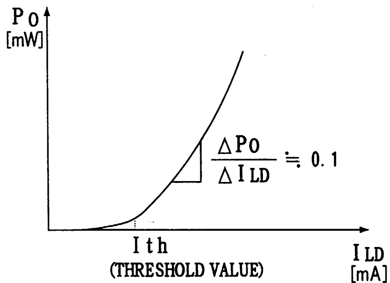
FIG.15 PRIOR ART
