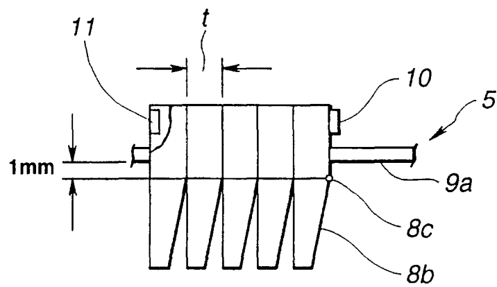
FIG.10 (PRIOR ART)
