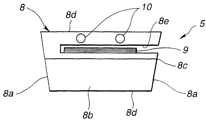
FIG.9 (PRIOR ART)
