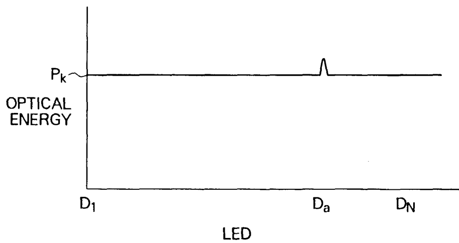
FIG. 4 PRIOR ART
