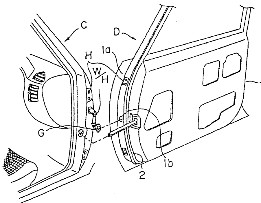
FIG. 39 PRIOR ART
